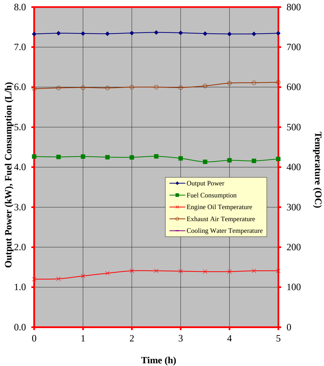
Figure 4. Performance characteristic curves during the continuous running test of the HONDA GX390H1 QP gasoline engine
