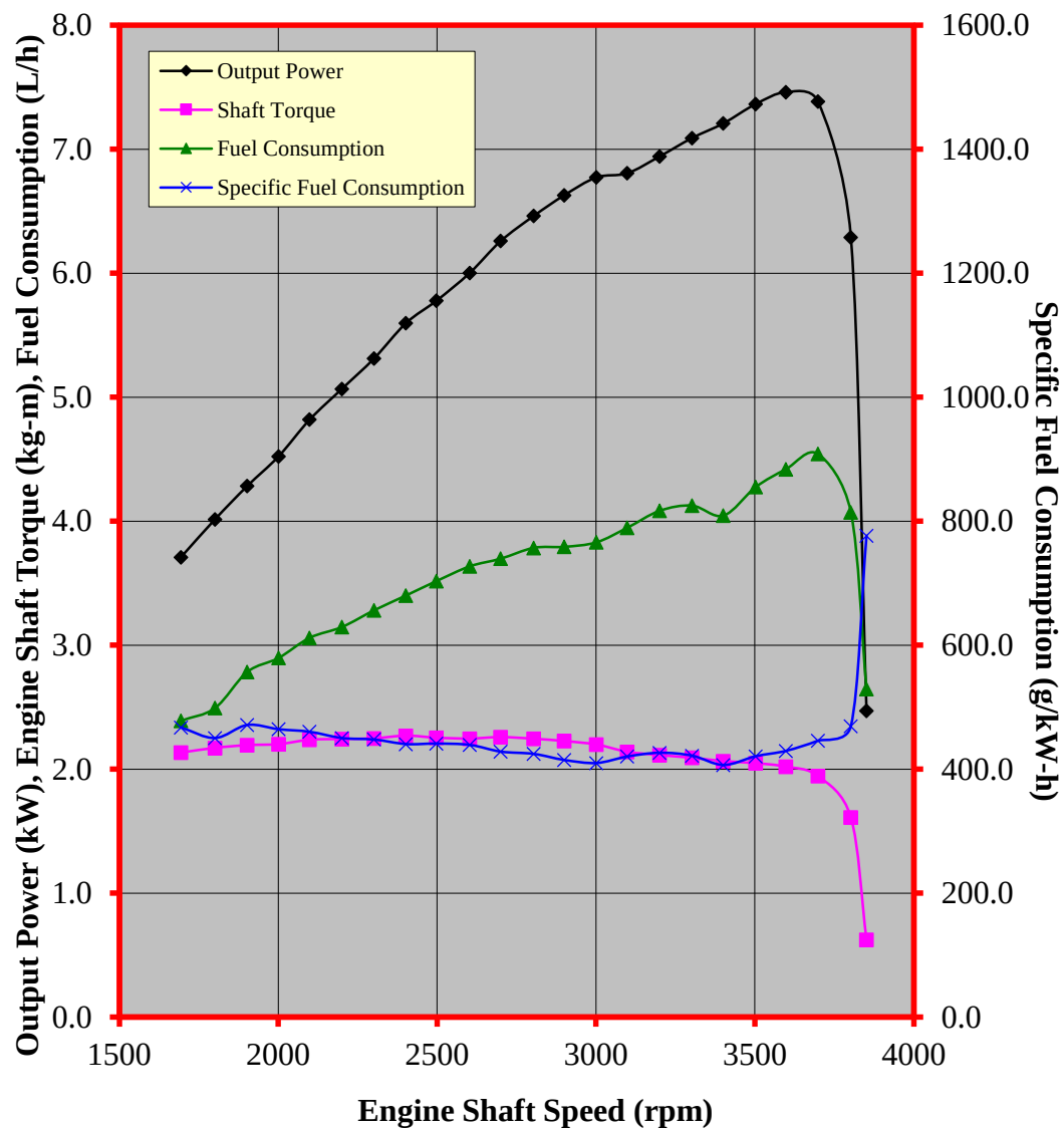
Figure 3. Performance characteristic curves of the HONDA GX390H1 QP gasoline engine
